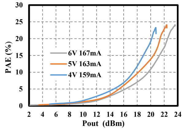
Figure 9. PAE vs. Pout @ 34GHz
