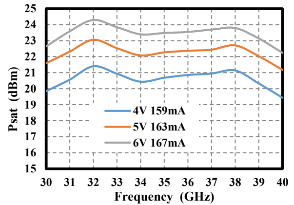
Figure 11. Psat vs. Vd
