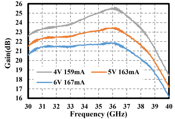
Figure 3. Gain vs. V_d
