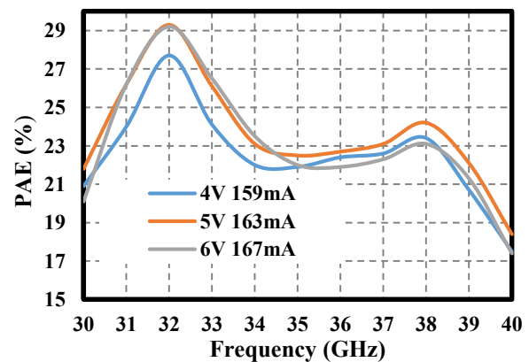
Figure 7. PAE vs. V_d
