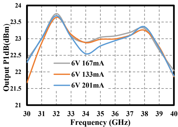
Figure 6. P1dB vs. I_d
