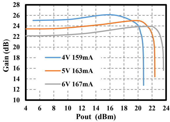
Figure 8. Gain vs. Pout @ 34GHz
